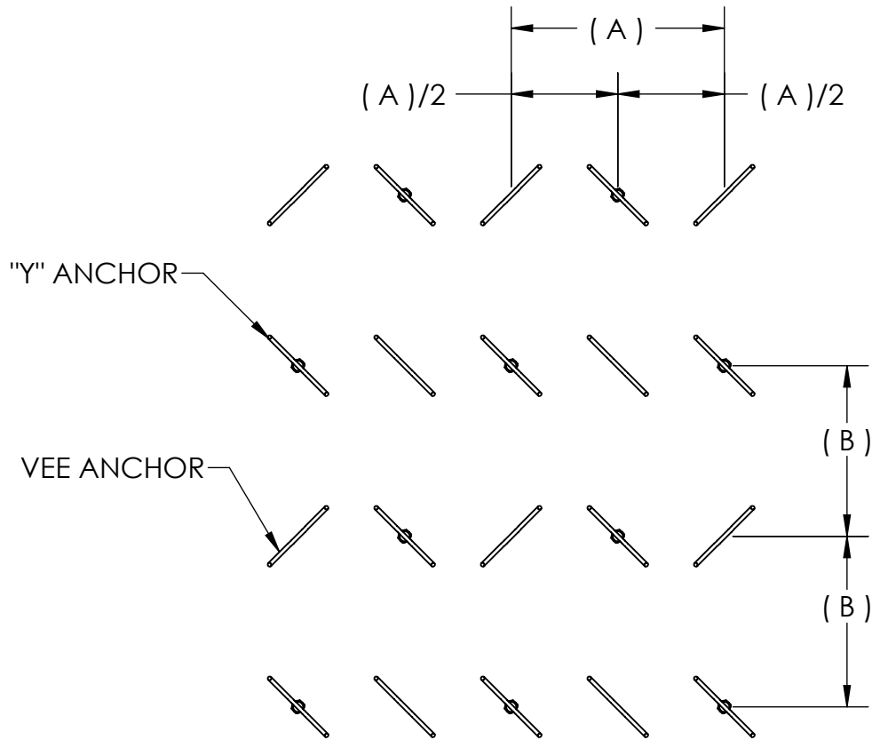
VEE AND "Y" ANCHOR INSTALLATION PATTERN
