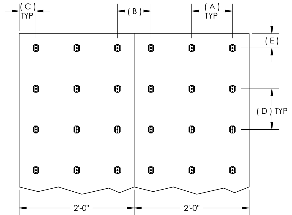
ROOF 24" WIDE BLANKET COMPRESSION JOINTS
