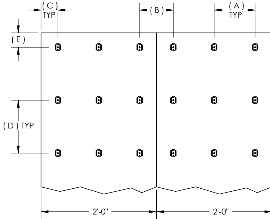
WALLS 24" WIDE BLANKET COMPRESSION JOINTS
